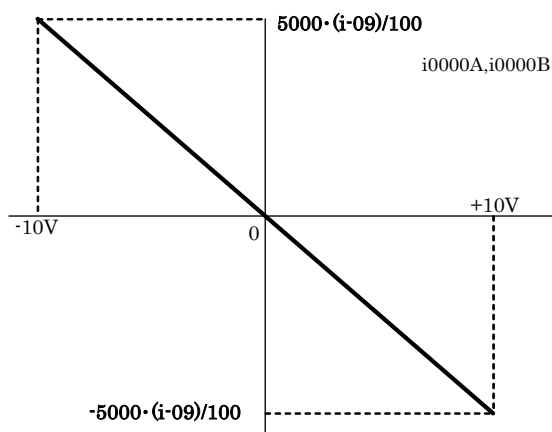
Input characteristic(0~±10V)
