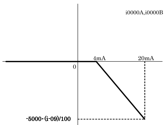
Input characteristic(4~20mA)
