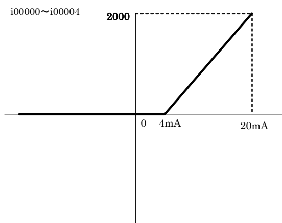
Input characteristic(4~20mA)
