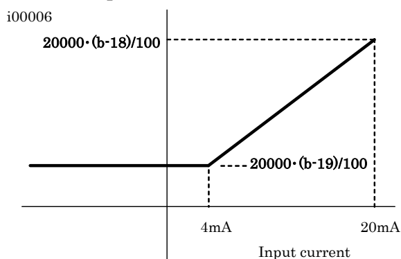
Lower limit speed(b-19)-positive Input characteristic(4~20mA)
