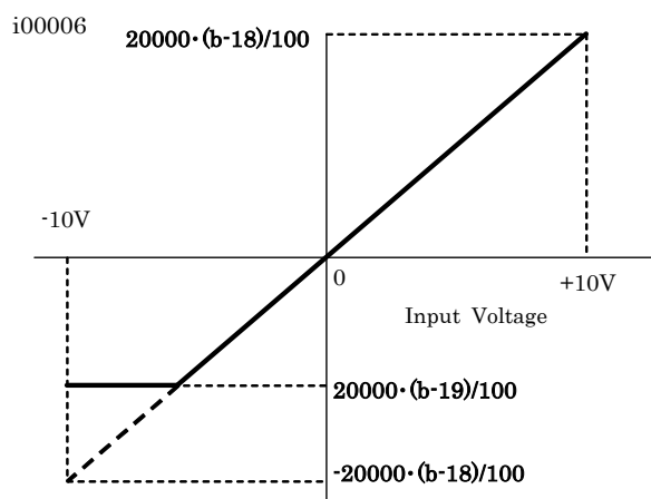
Input characteristic(0~±10V)
