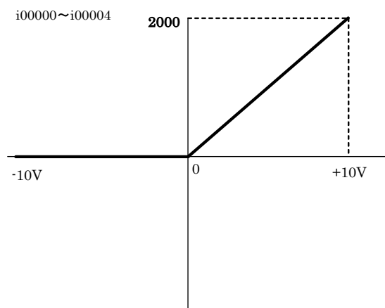
Input characteristic(0~10V)
