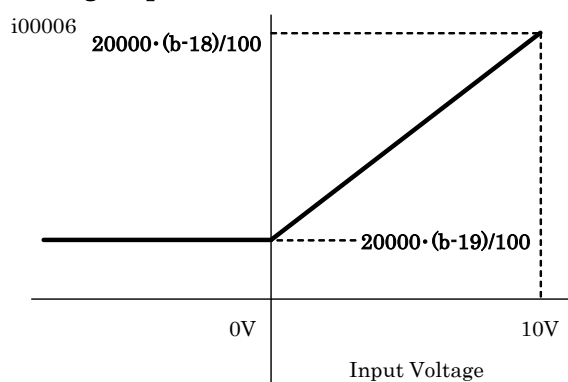
Lower limit speed(b-19)-positive Input characteristic(0~10V)
