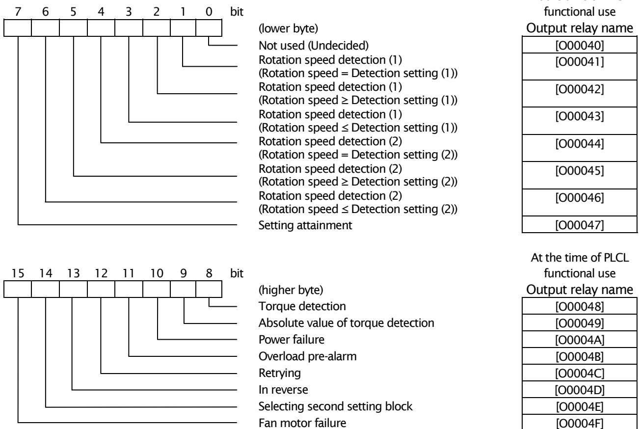
Figure 3.10 Bit configuration of 4th word
